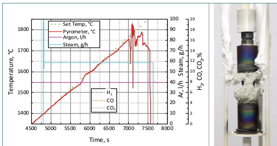
Figure 7. Conduct and results of the transient experiment with SiCf-SiC. Left: Temperature, gas/steam injection, and MS results for hydrogen, CO and CO 2 ; Right: Post-test appearance of the sample.
