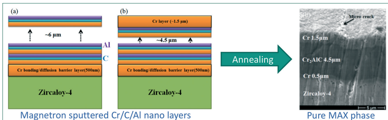
Figure 4. Synthesis of phase-pure Cr 2 AlC MAX phase coating on Zircaloy-4 substrate: 1) Magnetron sputtering with three element targets of nanoscale multilayer stacks and 2) subsequent annealing at 500°C in inert atmosphere.
