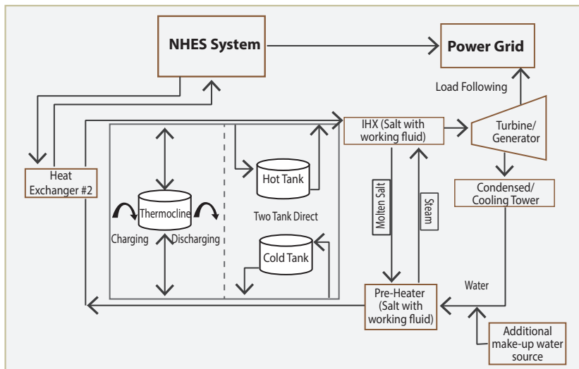
Figure 2. Molten salt ESS options.
