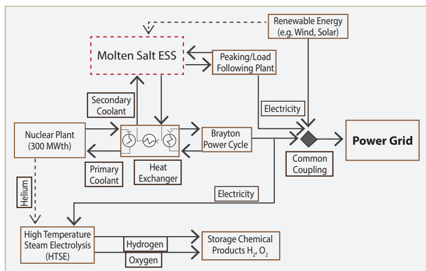
Figure 1. Nuclear hybrid energy system with a molten salt ESS.
