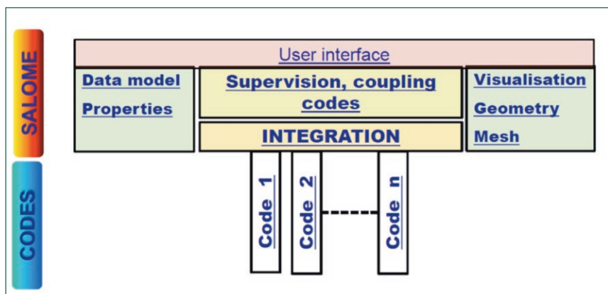
Figure 2. Architecture of the NURESIM platform.
