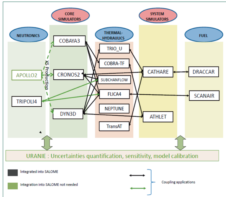
Figure 3. The NURESIM platform, at the end of the NURESIM project (January 2016).
