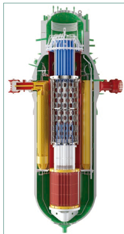
Figure 1. Reactor pressure vessel.
