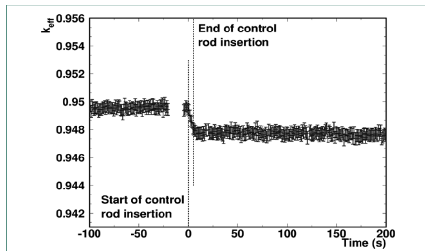
Figure 3. Measured values of the criticality constant ( k_{eff} ) of the YALINA-Booster subcritical assembly during a control rod insertion [17].
