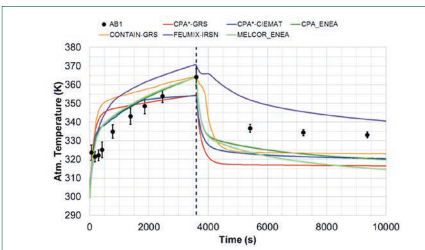
Figure 5. Atmosphere temperature (AB1).
