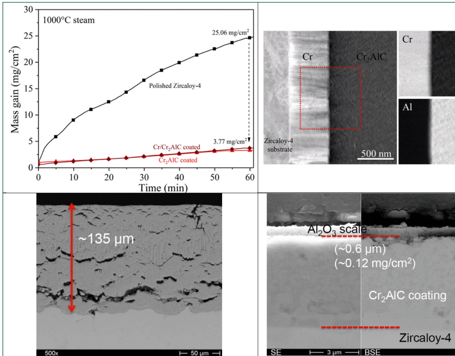
Figure 5. One hour oxidation of Cr 2 AlC on Zry-4 at 1000°C in steam; Top, left: TG curves of two coating design compared to non-coated Zry-4; Top, right: STEM image of Cr 2 AlC/Cr interface and corresponding EDS mapping before oxidation; Bottom, left: SEM image of non-coated Zry-4 reference sample, Bottom, right: SEM image of coated sample after oxidation.
